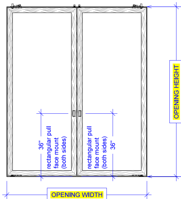
ELEVATION: closed
