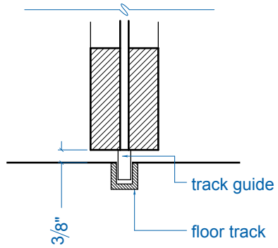
Sliding or Folding Door with floor track
