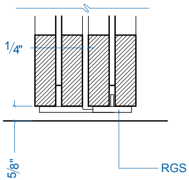
Sliding Wall
