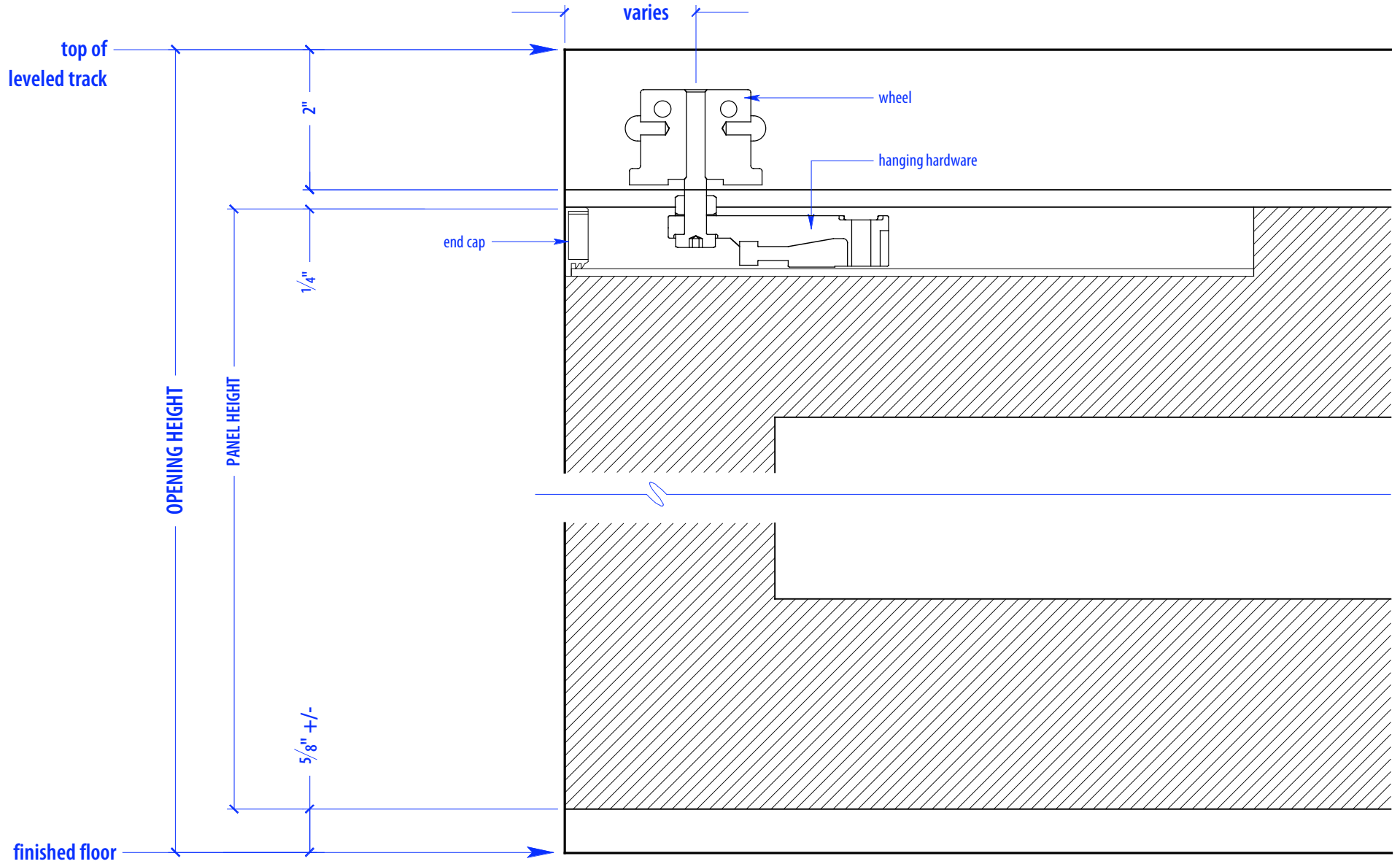
DETAIL B
