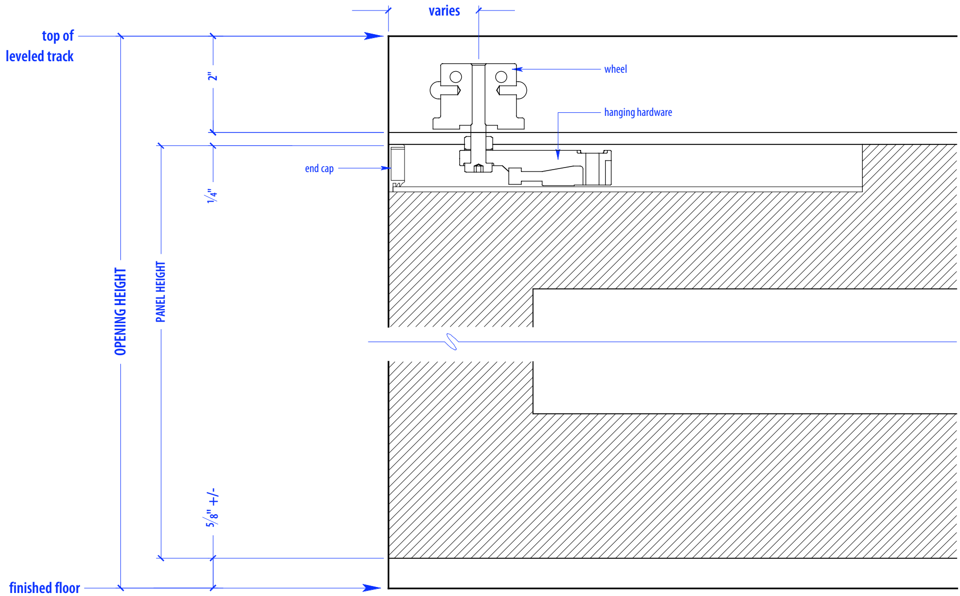
DETAIL B
