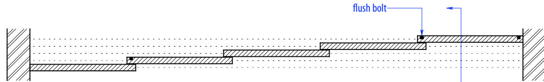
PLAN closed
