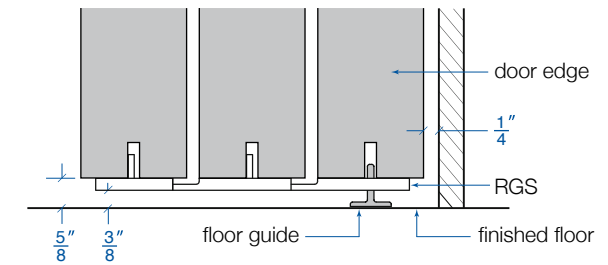
(SWW) Sliding Wing Wall
