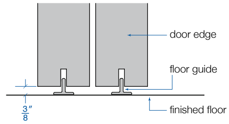
(SB) Sliding Bypassing
