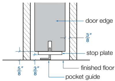
(SP) Sliding Pocket
