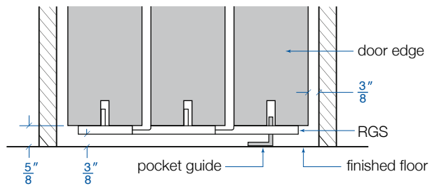
(SPW) Sliding Pocket Wall
