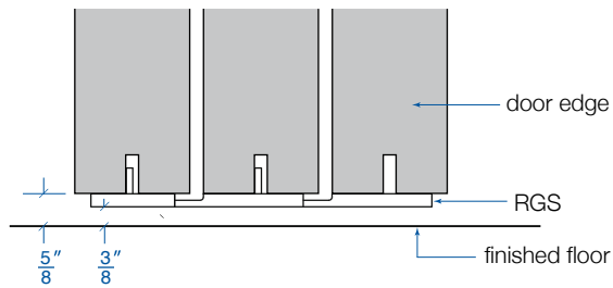
(SW) Sliding Wall
