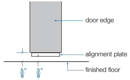
(SSPA) Sliding Stacking Parallel
