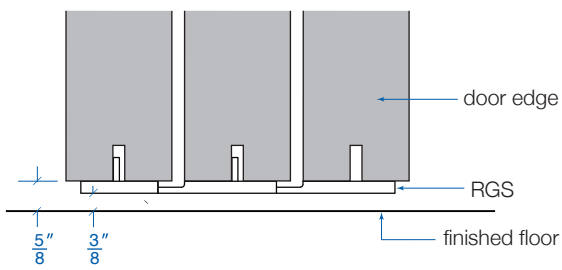
(SW) Sliding Wall pg. 13
