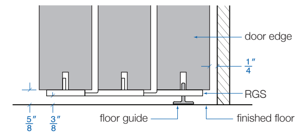
(SWW) Sliding Wing Wall pg. 15
