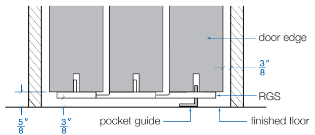
(SPW) Sliding Pocket Wall pg. 19
