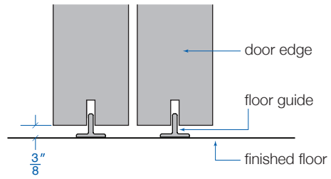
(SB) Sliding Bypassing pg. 11
