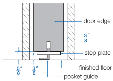
(SP) Sliding Pocket pg. 17
