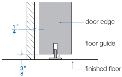
(S) Sliding pg. 9
