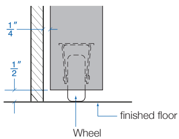
(SR) Sliding Rolling
